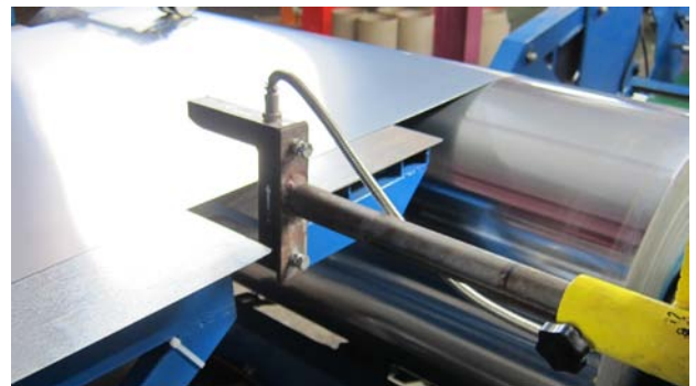
Infrared Sensor DS-100 is used on a Steel Web Finishing Machine
